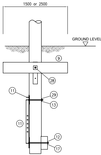
SECTION 3 Scale 1:25
